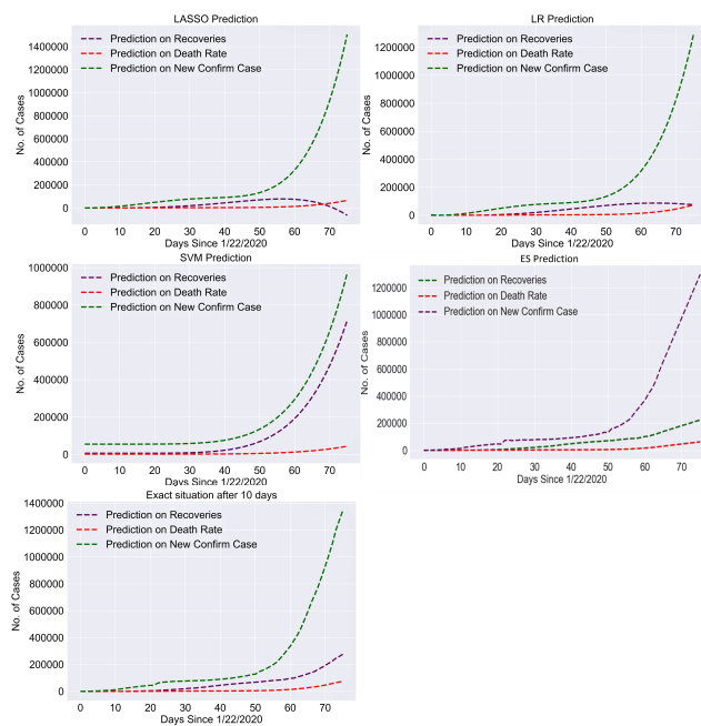
FIGURE 19: All models predictions from 1/22/2020 to 4/6/2020 and real situation from 1/22/2020 to 4/6/2020
